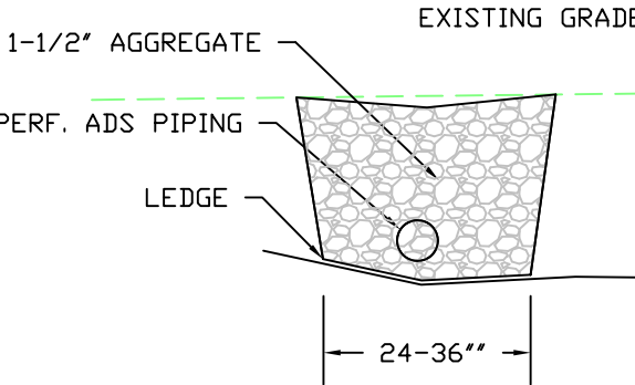
SUB-DRAIN DETAIL
