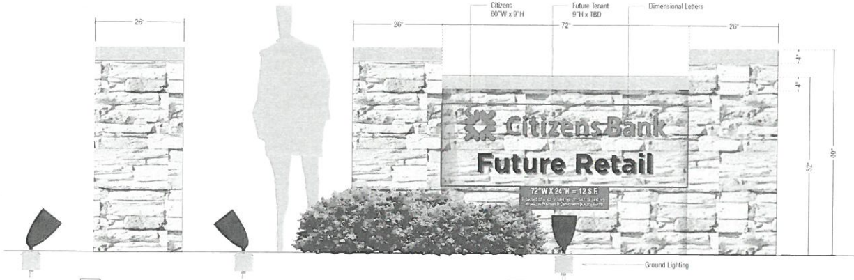
2 End View Scale: 1:4 Fabrication
