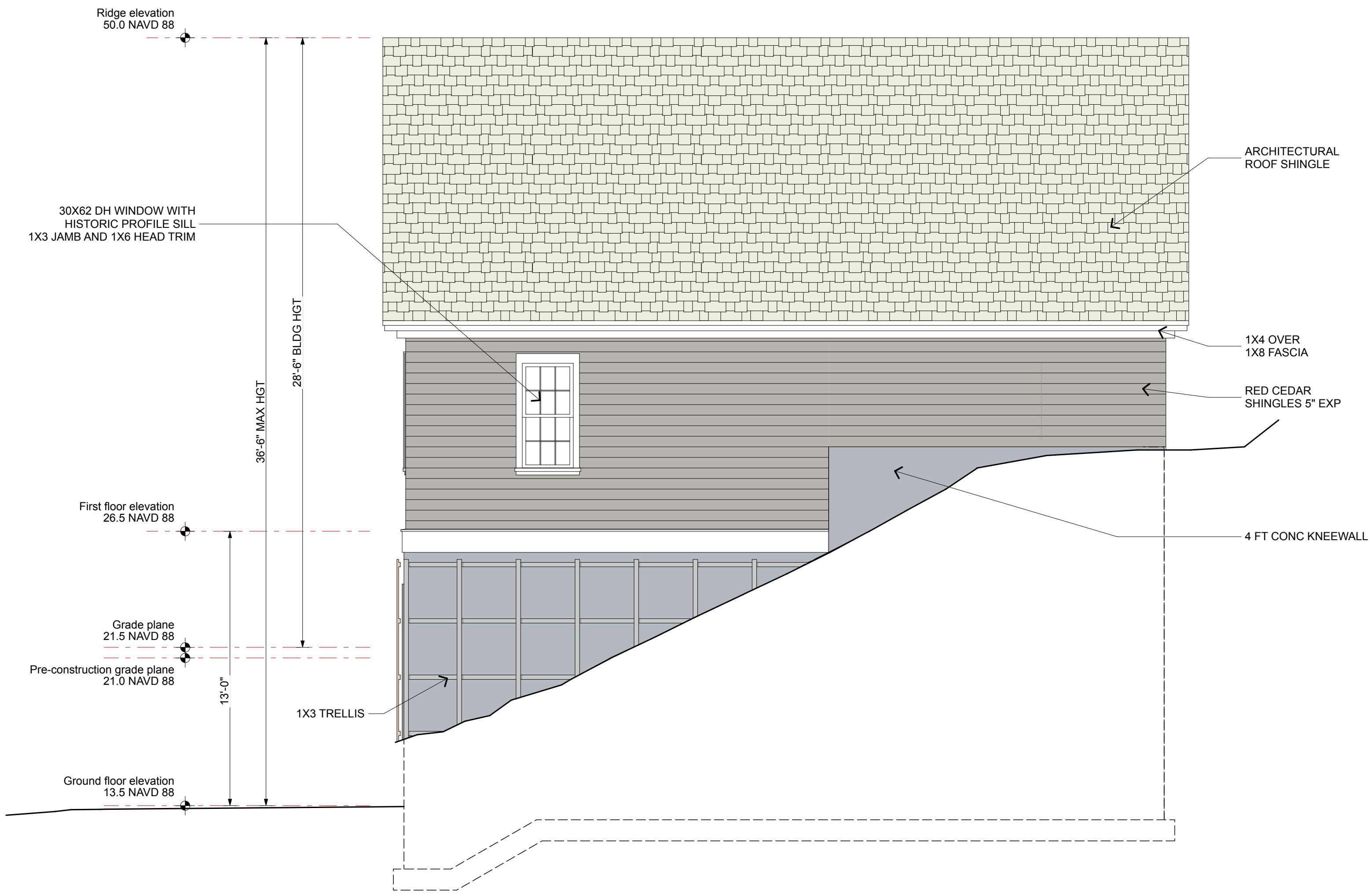
2 Building Elevation - North SCALE: 1/4" = 1'-0"
