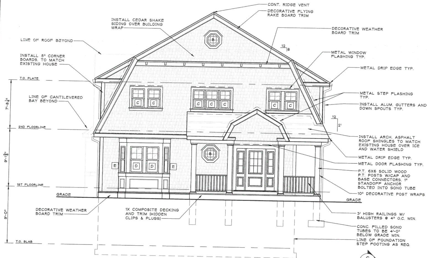
A FRONT ELEVATION A-2A SCALE 1/4"=1'-0"
