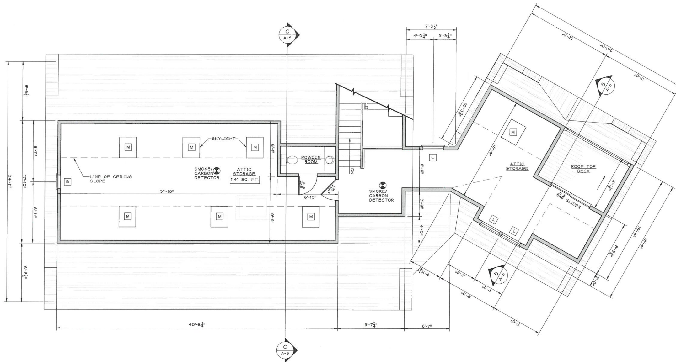
A ATTIC STORAGE PLAN A-IC SCALE: 1/4"=1'-0"
