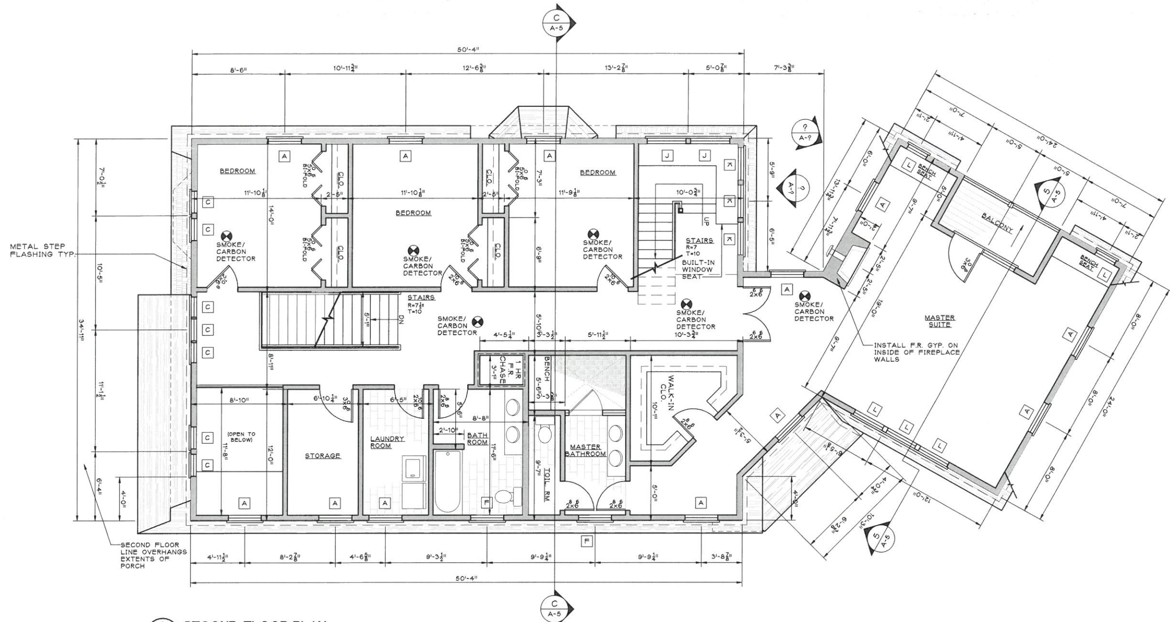
A SECOND FLOOR PLAN A-B SCALE: 1/4"=1'-0"
