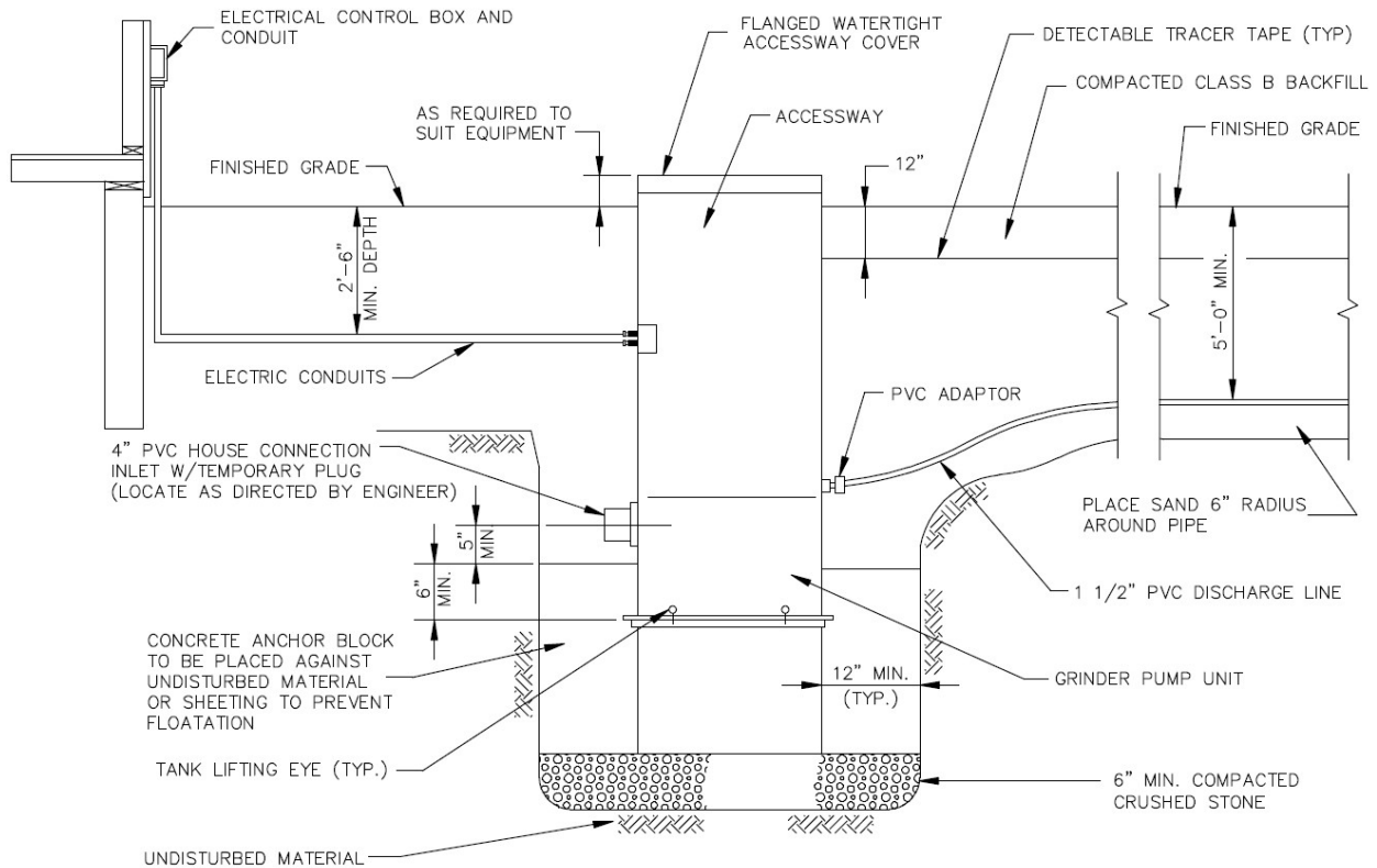
TYPICAL GRINDER PUMP INSTALLATION N.T.S.
