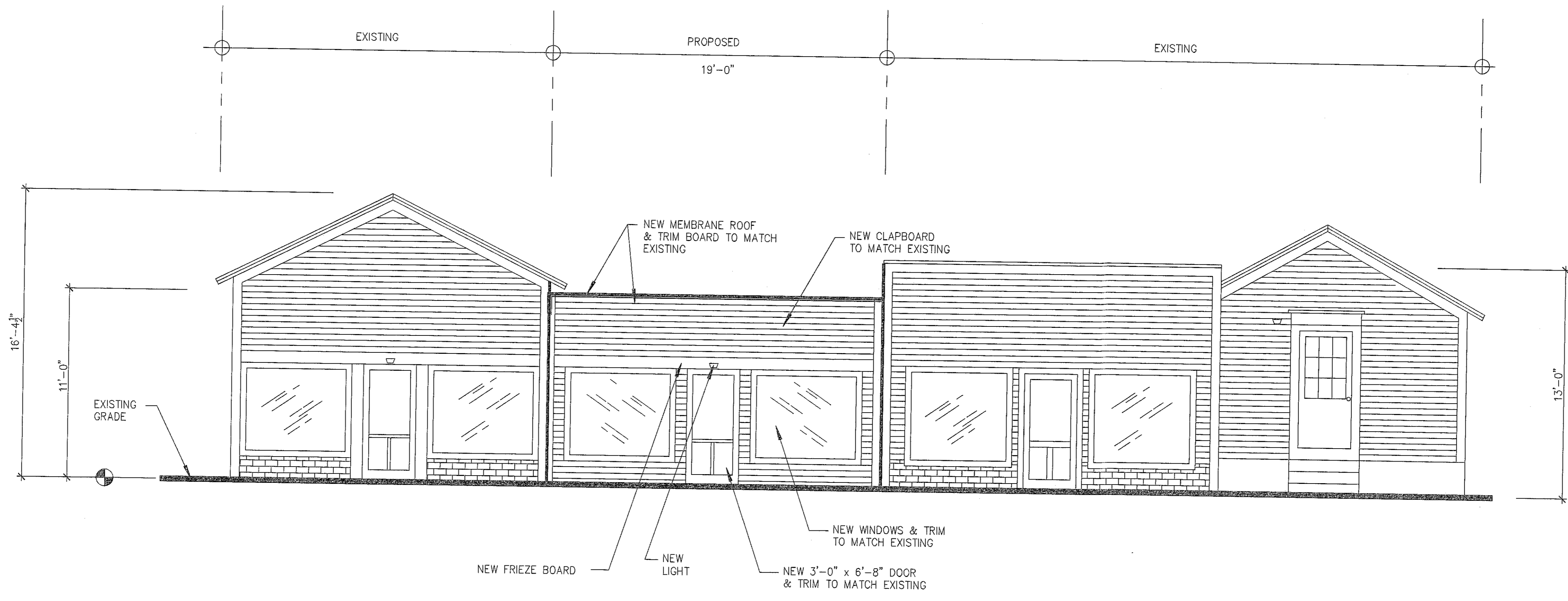
PROPOSED SOUTH STREET ELEVATION SCALE: 1/4" = 1'-0"
